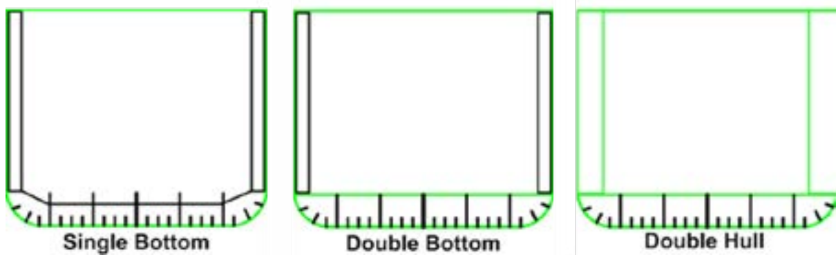
Figure 6-4. The double hull configuration.
