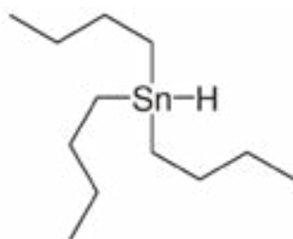
Figure 2-38. Tributyltin
