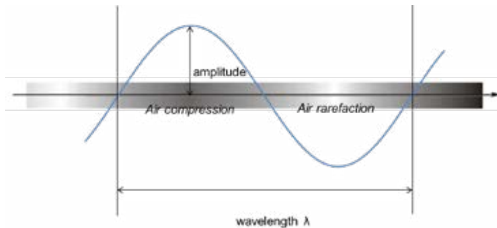
Figure 5-7. A travelling sound wave has amplitude and pitch.
