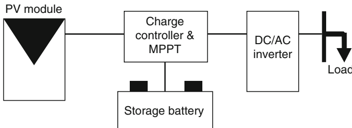
Fig. 4.23 Typical PV system components
