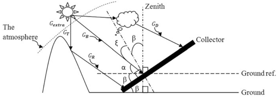
Fig. 4.2 Radiation components of solar energy on a collector with tilted surface
