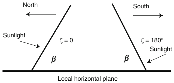
Fig. 4.5 Two solar collectors with different azimuths but with the same elevation
