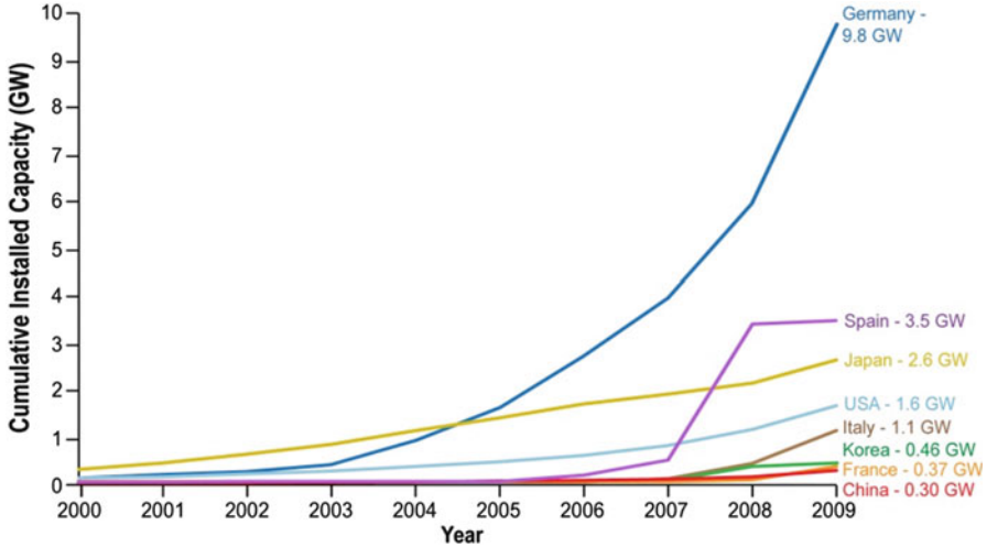
Fig. 4.6 PV cumulative installations [24]
