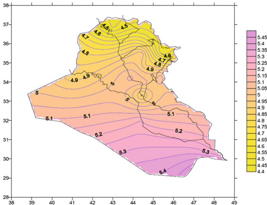
Fig. 2.5 The daily average solar insolation for different locations in Iraq
