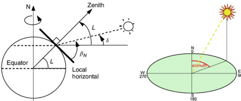
Fig. 4.3 Solar zenith angle
