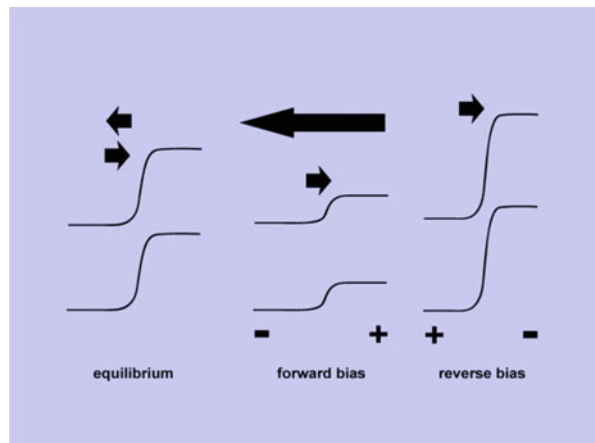
Fig. 4.12 Barriers charges
