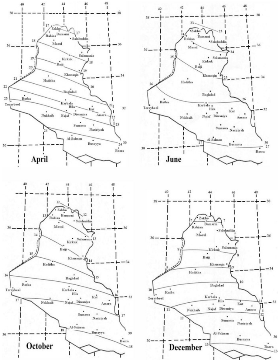
Fig. 3.3 Solar radiation lines for other months of Iraq [25]
