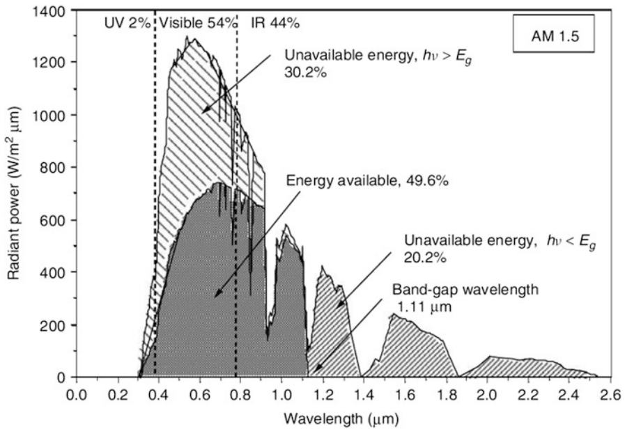
Fig. 4.13 Solar spectrum [25]
