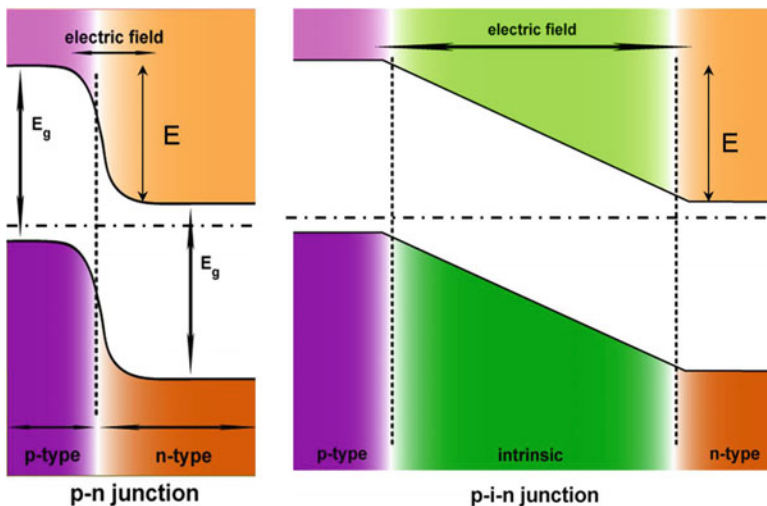
Fig. 4.11 “p-n” and “p-i-n” junctions
