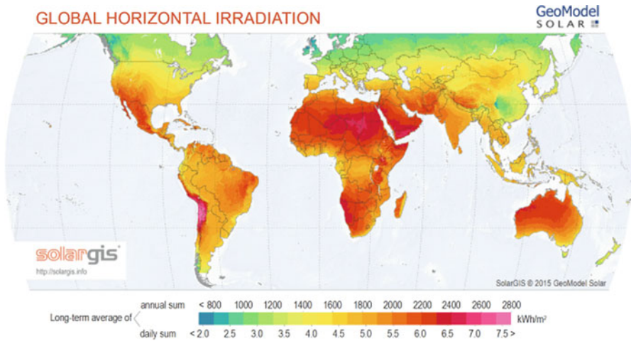
Fig. 1.3 Global solar irradiation map [21]
