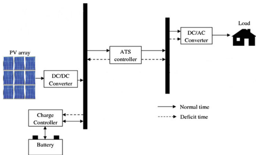
Fig. 4.19 Stand-alone PV system
