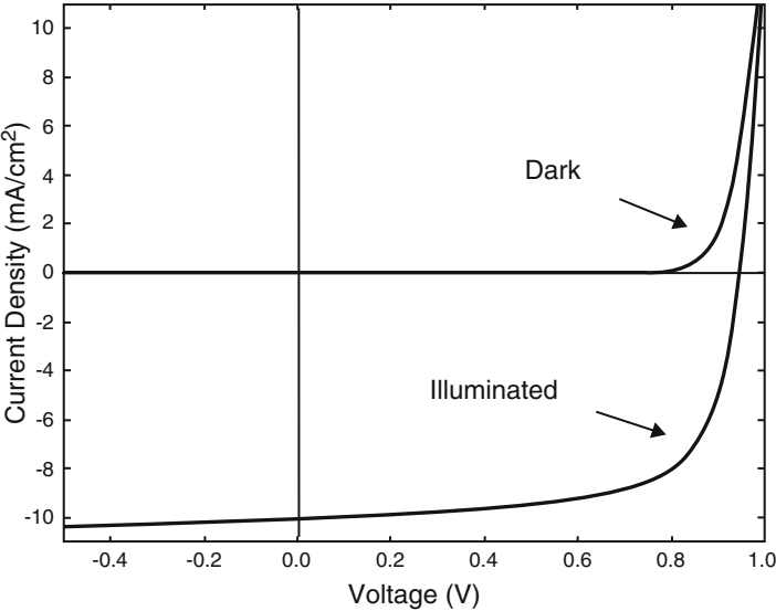
Fig. 4.15 Typical “ I - V characteristics”.
