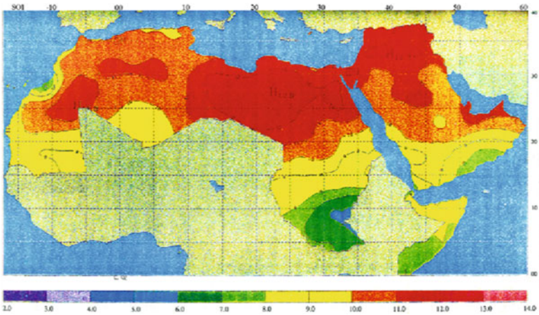
Fig. 5.2 The monthly average of the daily sunshine duration in hours for June in Arab countries [64]
