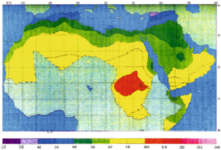
Fig. 5.1 The monthly average of the daily sunshine duration in hours for January in Arab countries [64]
